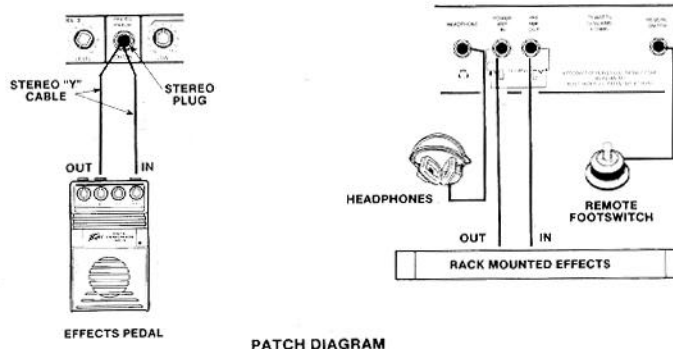
PATCH DIAGRAM
